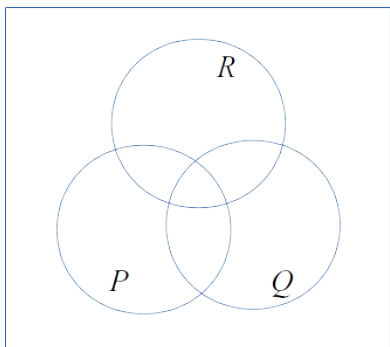
Figure 1. Venn diagram for 3 sets.
