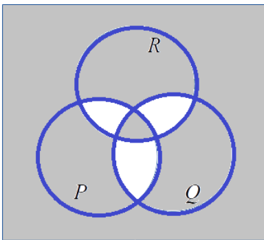
Figure 3. Venn diagram with shading.
